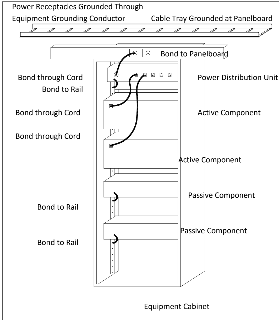
Figure 1. - Information Technology Equipment Rack Grounding
