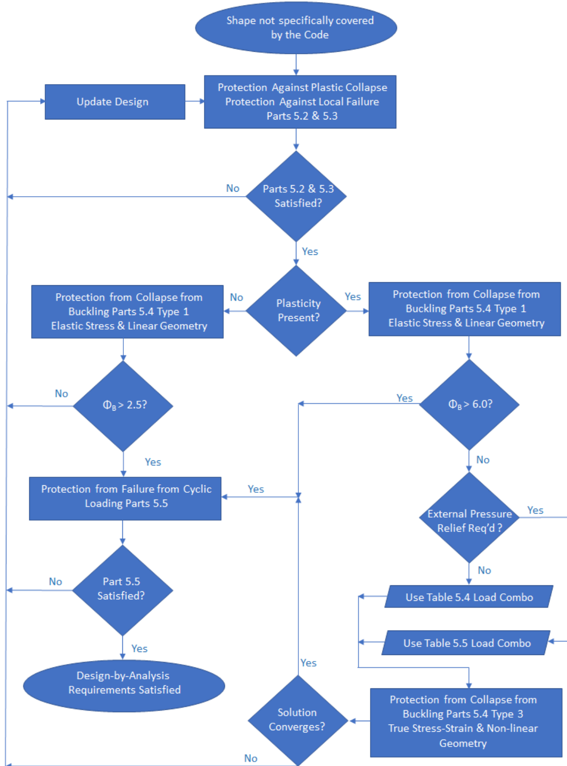
Figure 1: Flowchart describing the design-by-analysis process for shapes not specifically covered by ASME BVPC VIII
